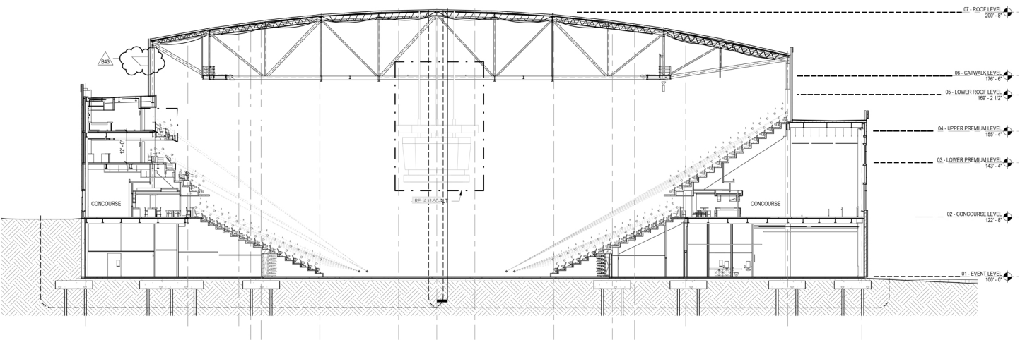
TRANSVERSE SECTION 1" = 0'
