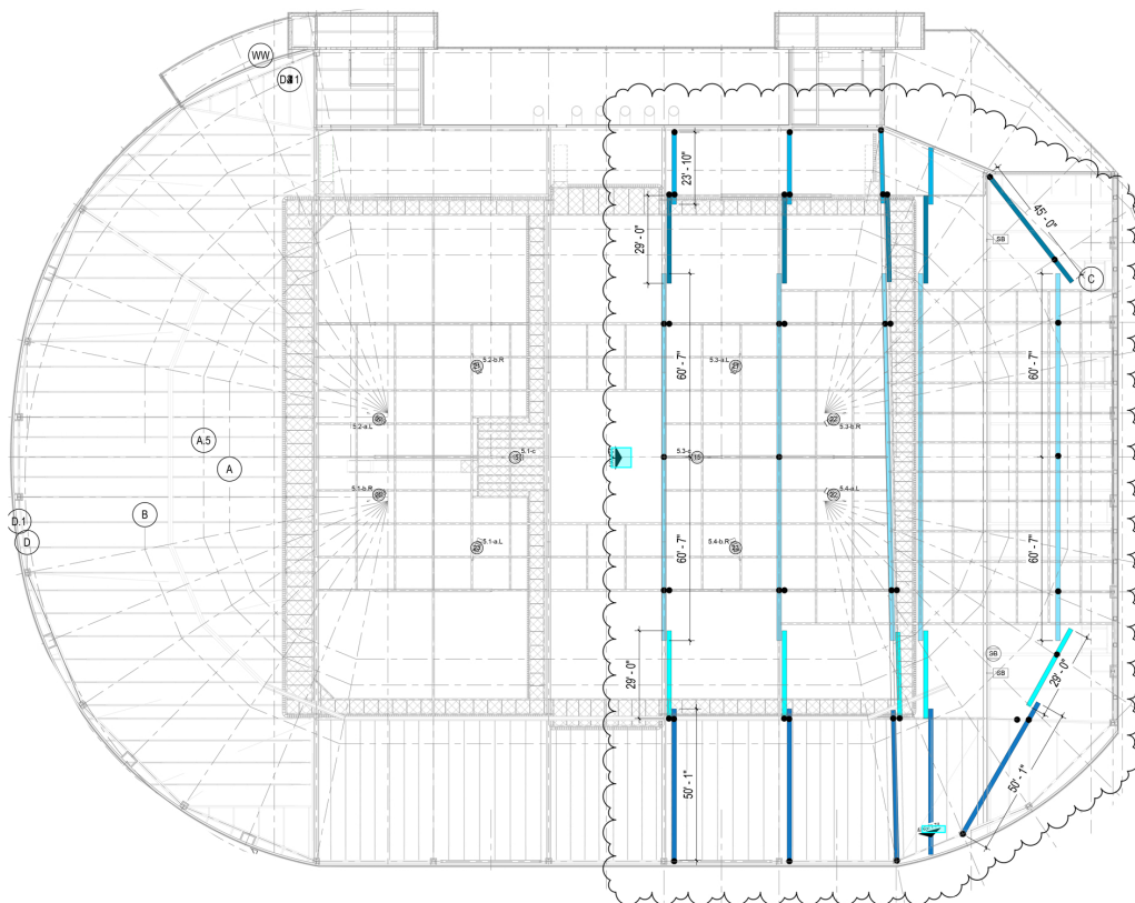
1 HALF HOUSE REDUCTION CURTAINS -OVERALL RCP
